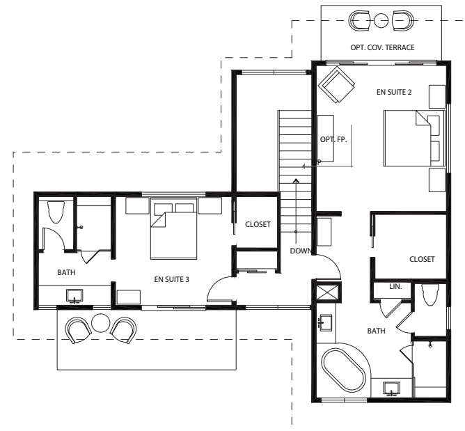
UPPER LEVEL
